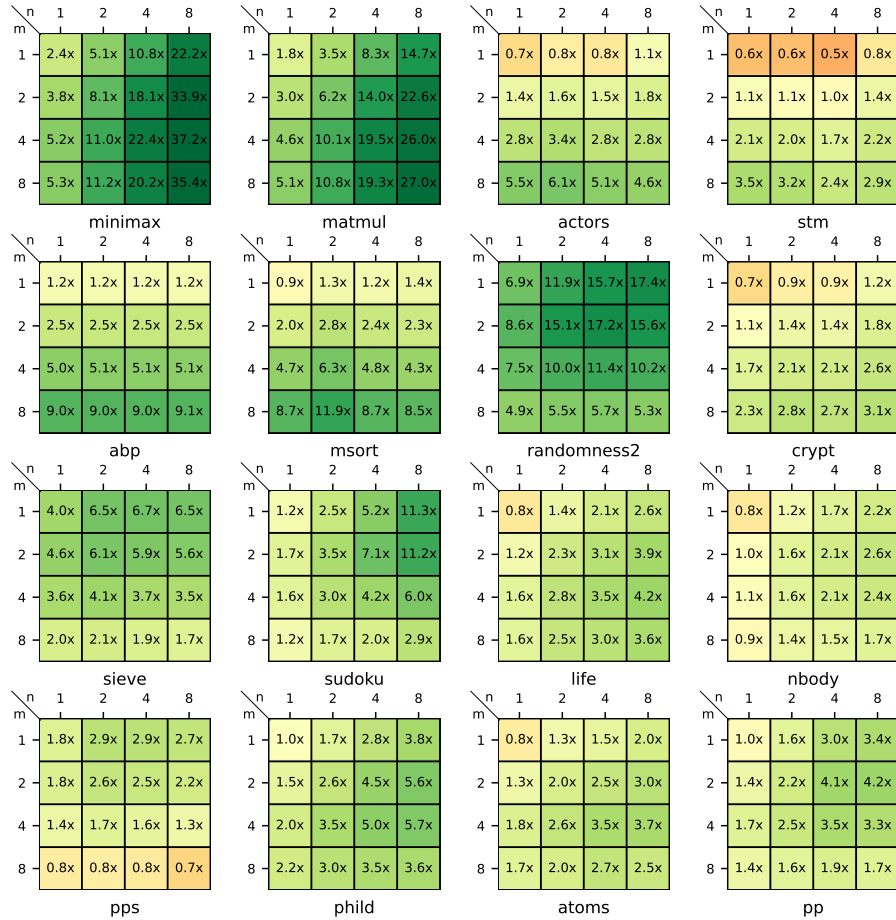
Figure 6: Speedups for the context-sensitive 5-CFA MODCONC analysis, relative to the sequential implementation. Horizontally (left-to-right), we increase the number of workers for MODCONC inter-component analysis. Vertically (top-to-bottom), we increase the number of workers per intra-component (MODF) analysis. Color is used to emphasise the magnitude of the speedup (or in some cases, slowdown).
