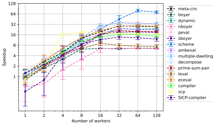
Figure 3: Speedups for the context-insensitive MODF analysis.
