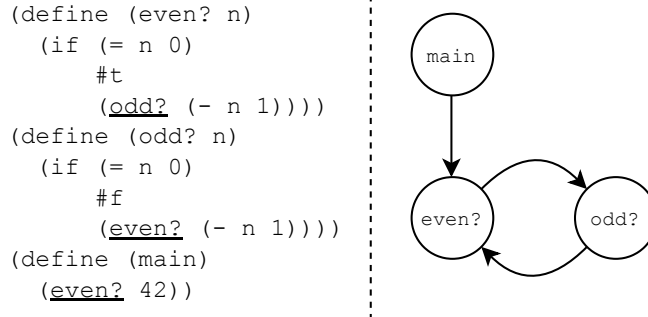
Figure 1: A MODF analysis example (left: the Scheme program under analysis; right: the call graph computed by a context-insensitive MODF analysis).
