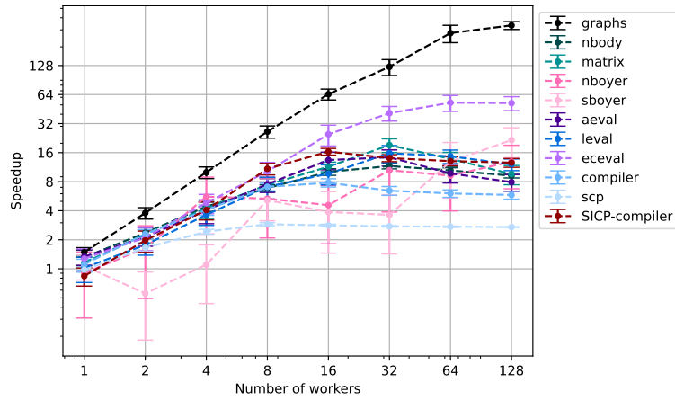
Figure 5: Speedups for the context-sensitive 2-CFA MODF analysis.
