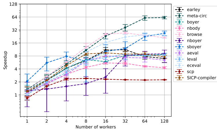
Figure 4: Speedups for the context-sensitive 1-CFA MODF analysis.
